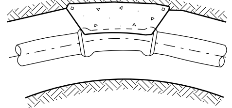
⑨ 11-1/4° & 22-1/2° BENDS
