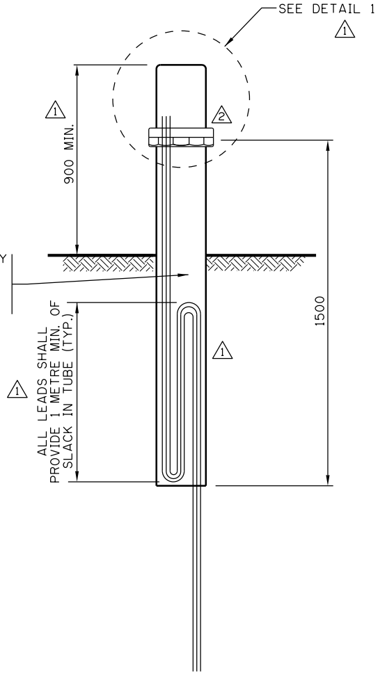
SECTION
