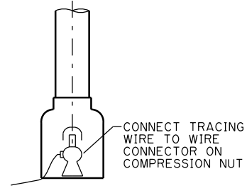
② CUL-DE-SAC TRACING WIRE DETAIL
