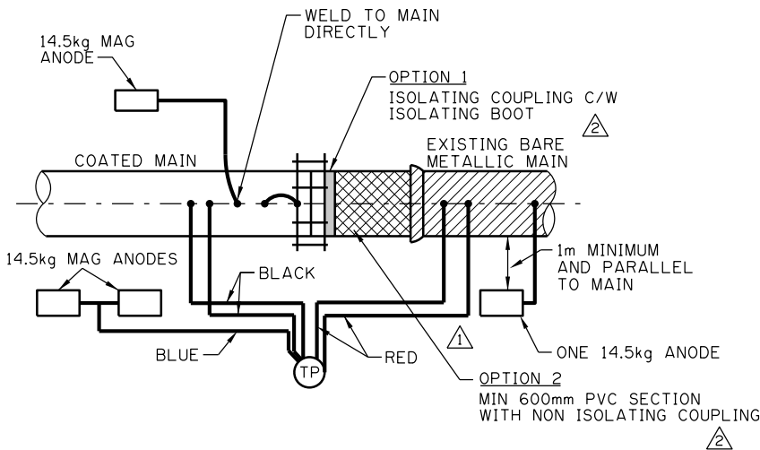
TYPICAL WIRE COLOUR DETAIL
