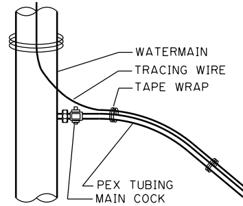
② CUL-DE-SAC TRACING WIRE DETAIL
