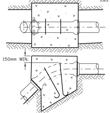
⑫ VERTICAL BEND - UP OR DOWN
