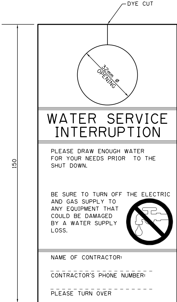
BACK SIDE
