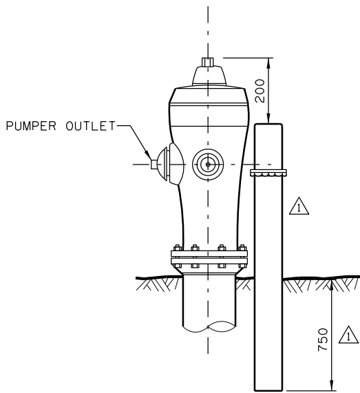
TEST POINT INSTALLATION AT A HYDRANT
