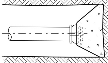
⑪ DEAD END
