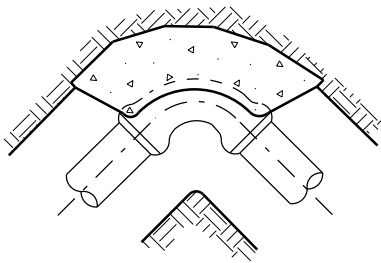
⑩ OFFSET BEND
