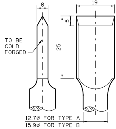
DETAIL B
