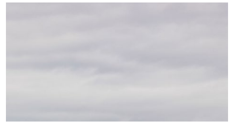
Cloudy
