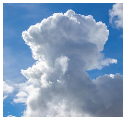
Cumulo-nimbus
