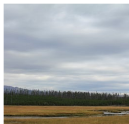
Stratus
