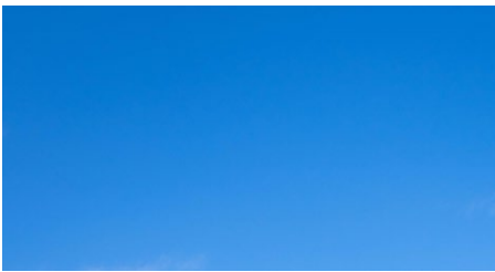
Clear skies
