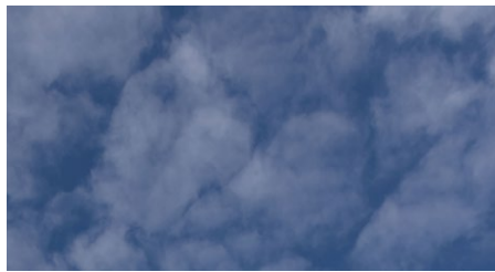
Partly cloudy
