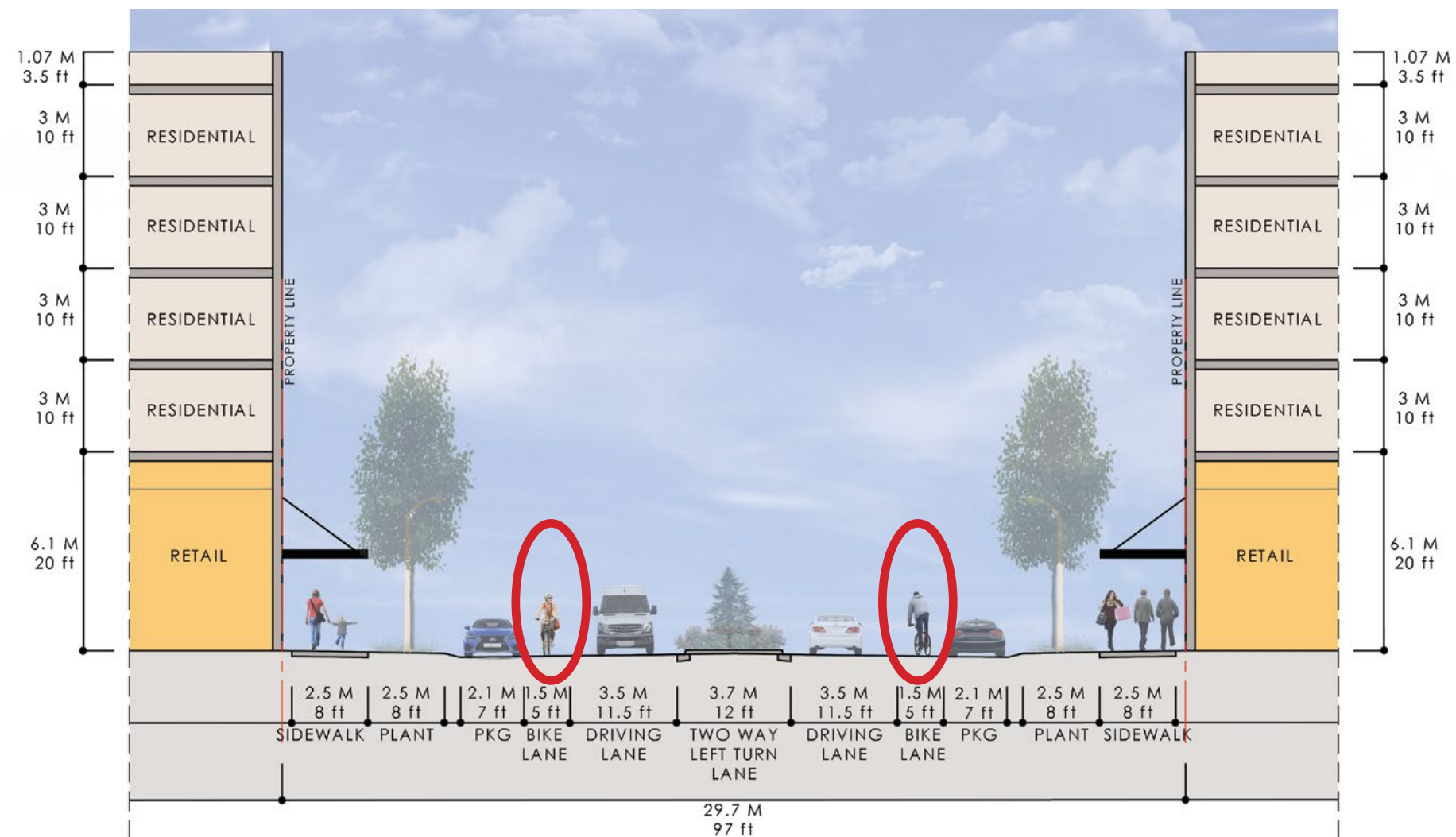
TOWN CENTRE STREET SECTION C-C' AS APPROVED BY CITY
