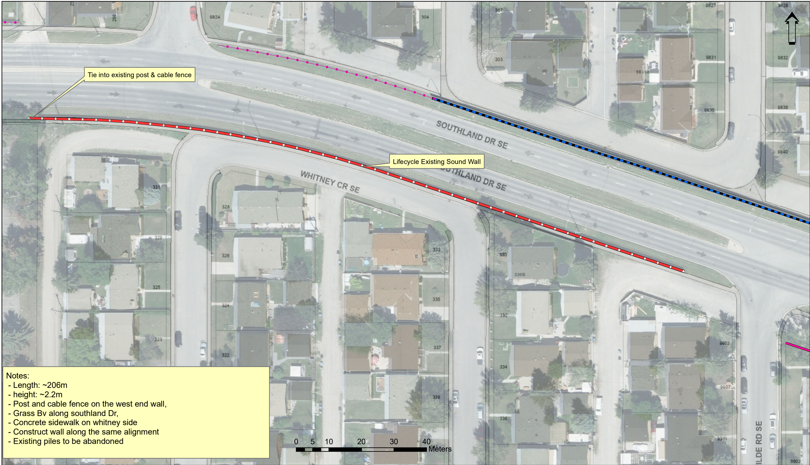
Location 7A: Southland Dr SE, West of Wilde Rd SE (Whitney Cr SE) - South Side Sound Wall Lifecycle Replacement Program
