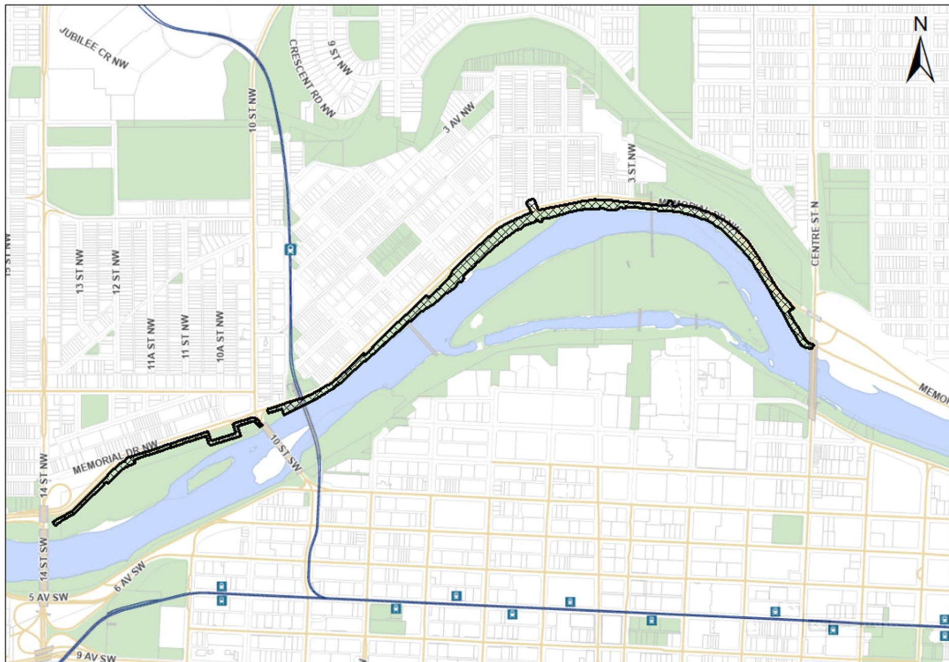
SUNNYSIDE FLOOD BARRIER PRE-CONSTRUCTION WORK AREAS
