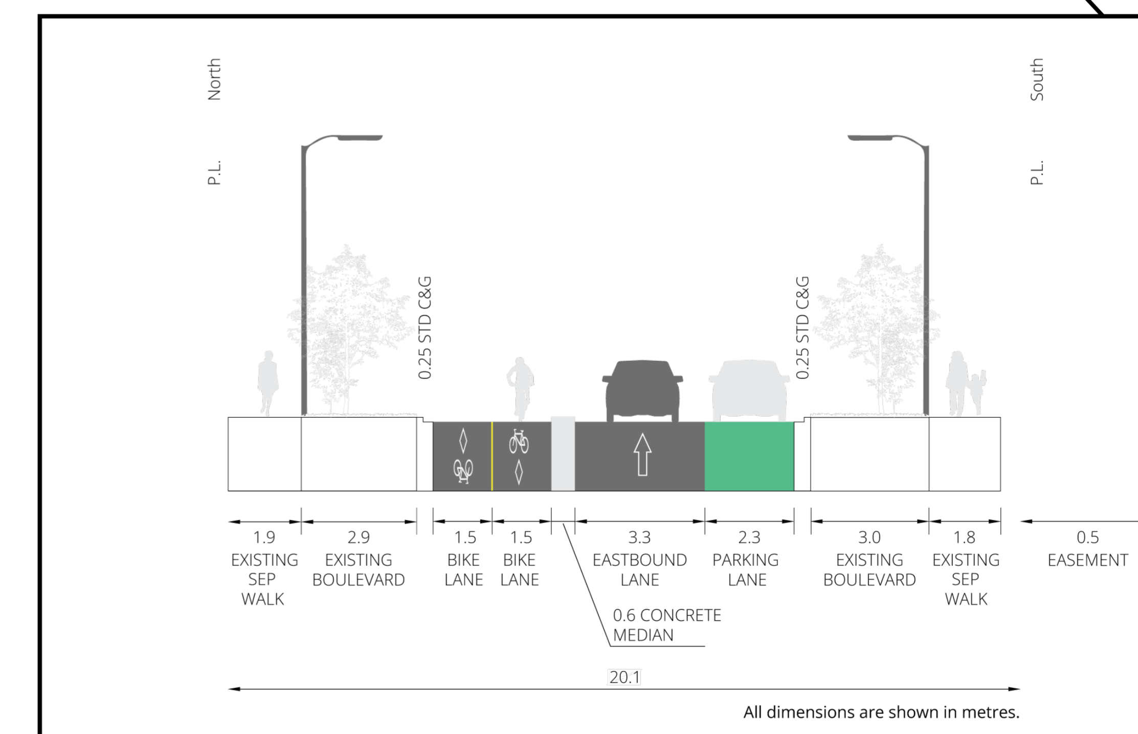
Cross Section A-A, 15 Avenue West of 10 Street SW
